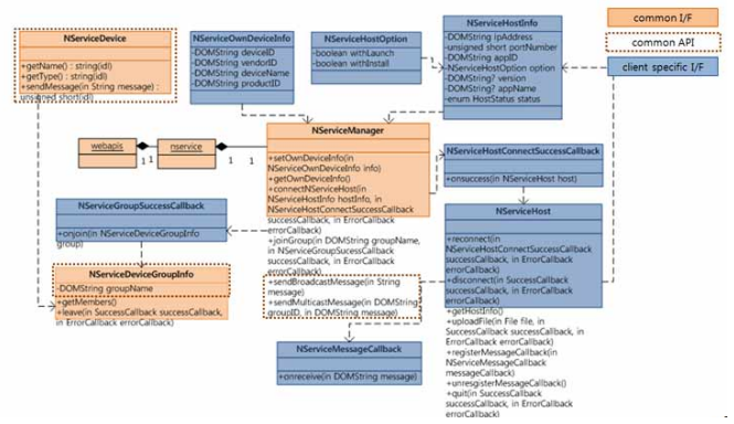
Figure 8: ER diagram of the N-Service API
